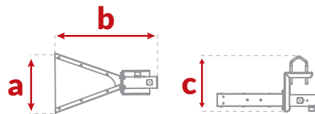
PD-5800-15-60-DP-ST5 PD-5800-15-60-DP-STN
